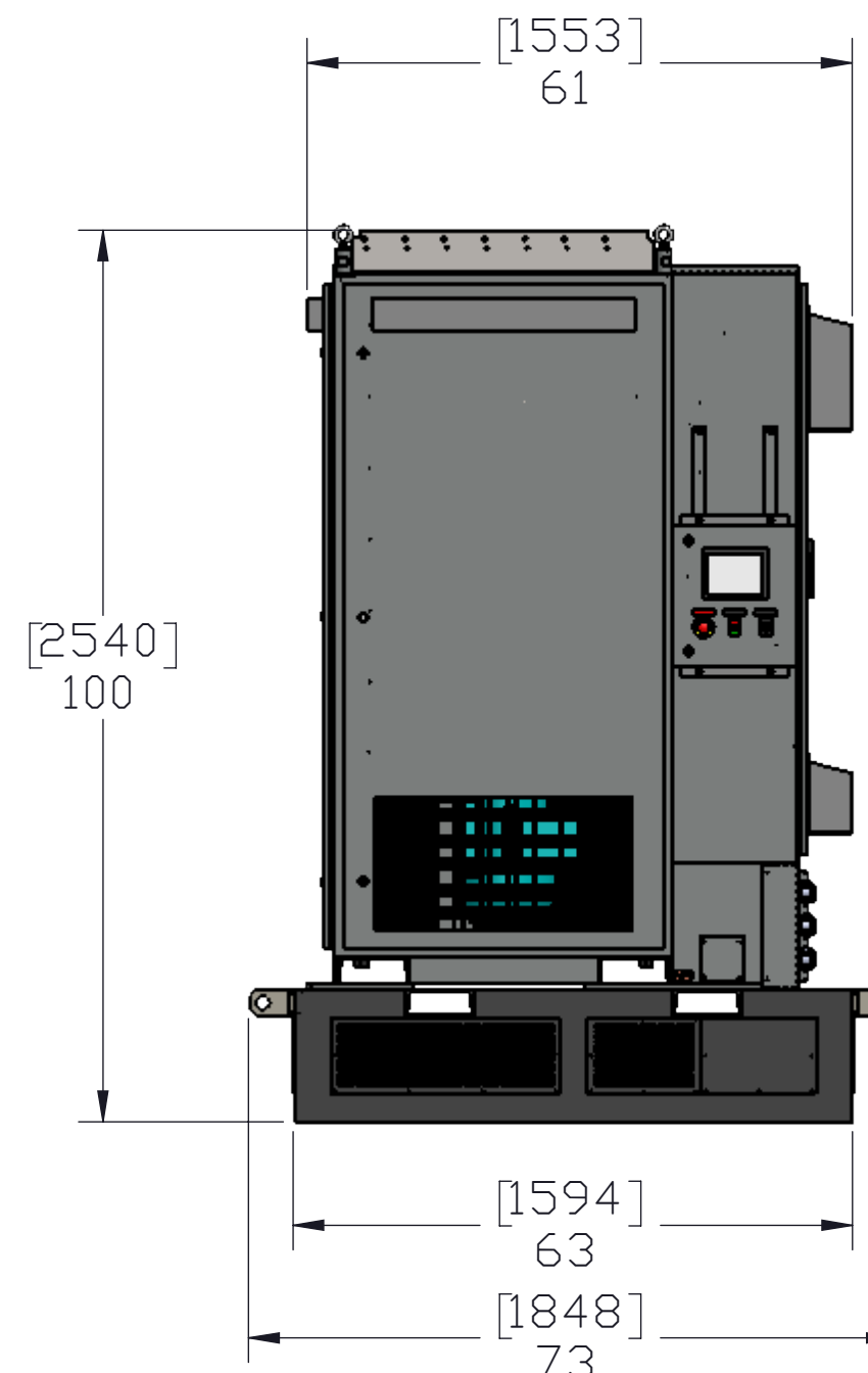
L.H.S VIEW
