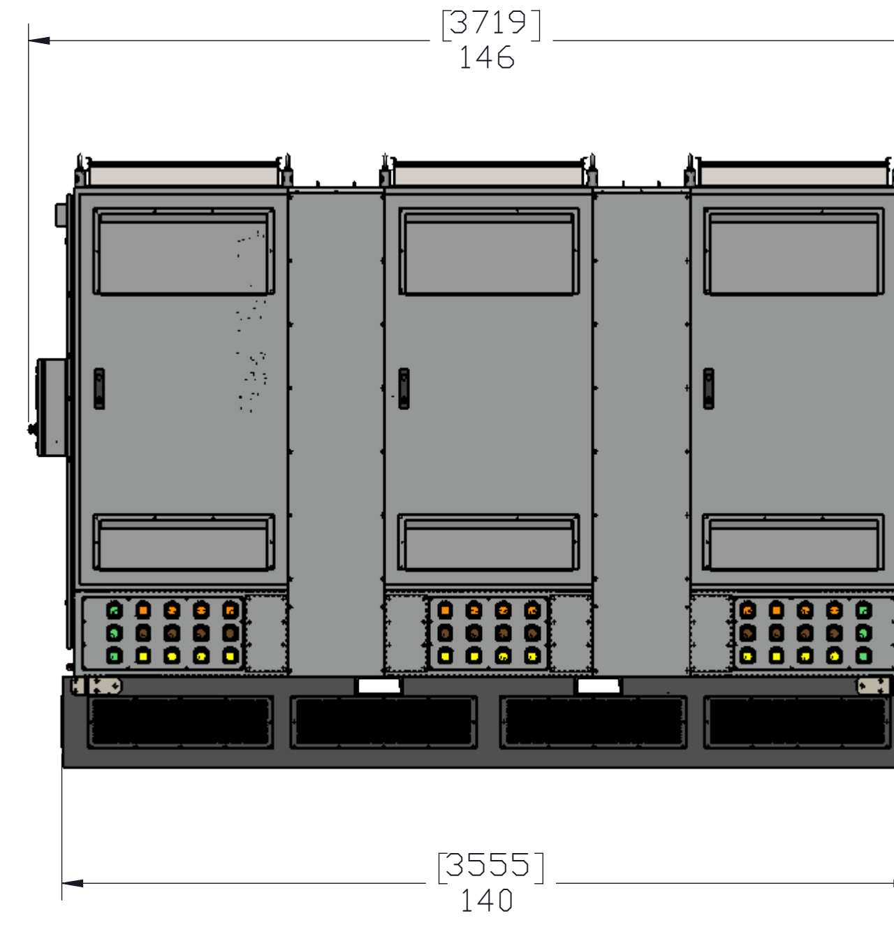
FRONT VIEW
